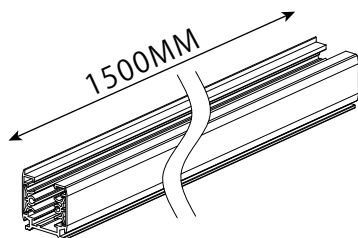
97692/106616 Max.loading 7.5kG
